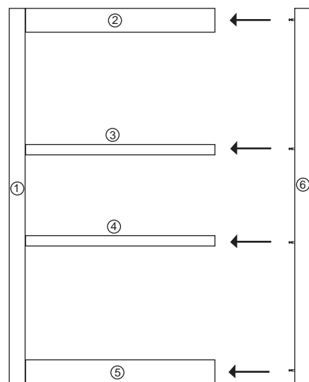
Attach side panel 6
